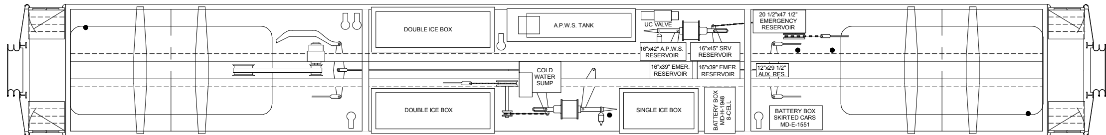
VIEW LOOKING UP FROM UNDERNEATH CAR
